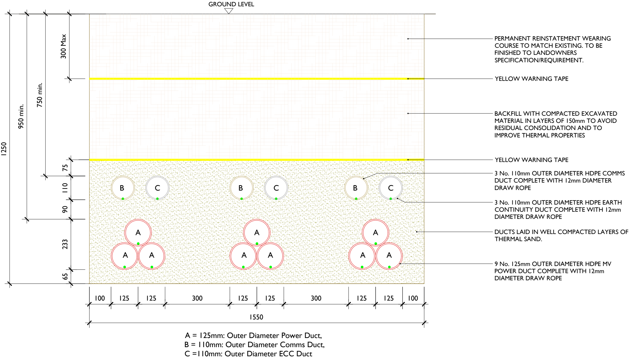
Typical Triple Circuit Section Through Grasslands SCALE 1:10
